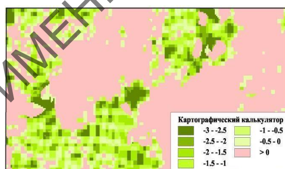
The result of arithmetic addition of grid- themes
