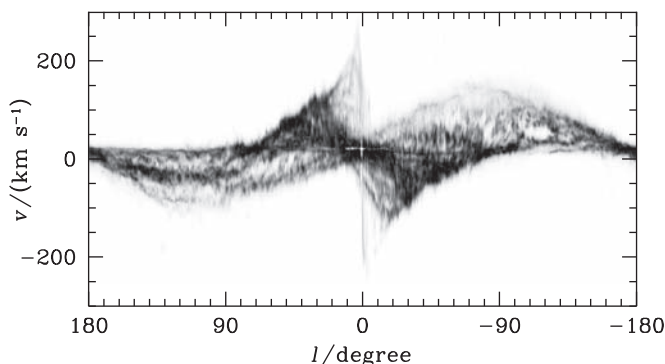
Fig. 6.8 The intensity I(l, b = 0^\circ, v_R) of the 21-cm line shown by grey scale in the l - v_R plane. As given by Binney and Merrifield (1998), based on the data provided by D. Hartmann. See Hartmann and Burton (1997) for details. Courtesy: D. Hartmann and M. Merrifield.
