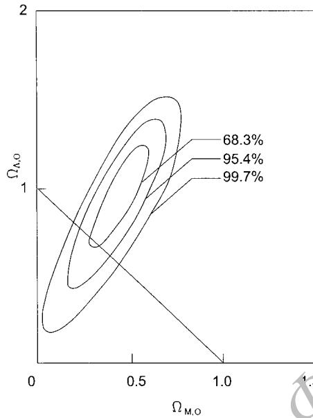
Fig. 14.6 Constraints on \Omega_{\Lambda,0} and \Omega_{M,0} jointly coming from the temperature anisotropies of the CMBR (the straight line corresponding to \Omega_{\Lambda,0} + \Omega_{M,0} = 1 ) and the data of distant Type Ia supernovae (the ellipses within which the values would lie at particular confidence levels). Adapted from Riess et al. (2004) .
