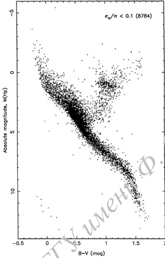
Fig. 3.5 The HR diagram (or colour–magnitude diagram) of nearby stars, constructed from the measurements by the Hipparcos astronomy satellite. From Perryman et al. (1995) . (©European Southern Observatory. Reproduced with permission from Astronomy and Astrophysics .)
