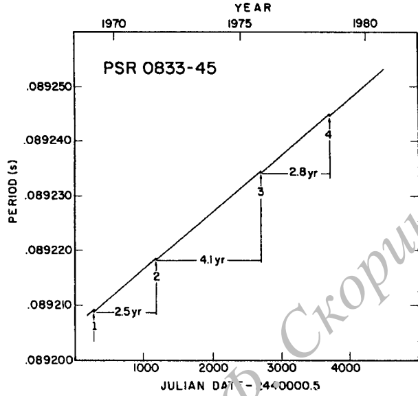
Fig. 5.4 Variation of the period of pulsar PSR 0833 – 45 from late 1968 to mid-1980. Four glitches are seen. From Downs (1981) . (©American Astronomical Society. Reproduced with permission from Astrophysical Journal .)
