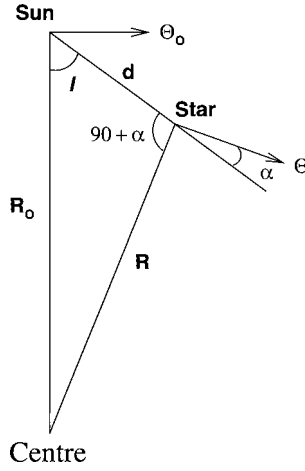
Fig. 6.4 A sketch indicating the Sun and a star going around the galactic centre.
