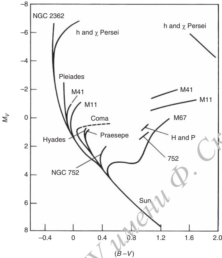
Fig. 3.9 A composite HR diagram, sketching the extent of the main sequence for several star clusters. From Sandage (1957). (©American Astronomical Society. Reproduced with permission from Astrophysical Journal .)
