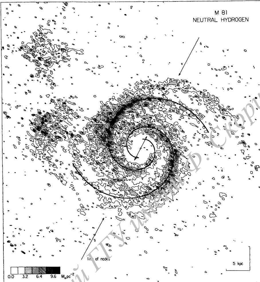
Fig. 8.7 The distribution of interstellar matter in the galaxy M81, as measured by radio emission from neutral hydrogen atoms. From Rots (1975) . (©European Southern Observatory. Reproduced with permission from Astronomy and Astrophysics .)
