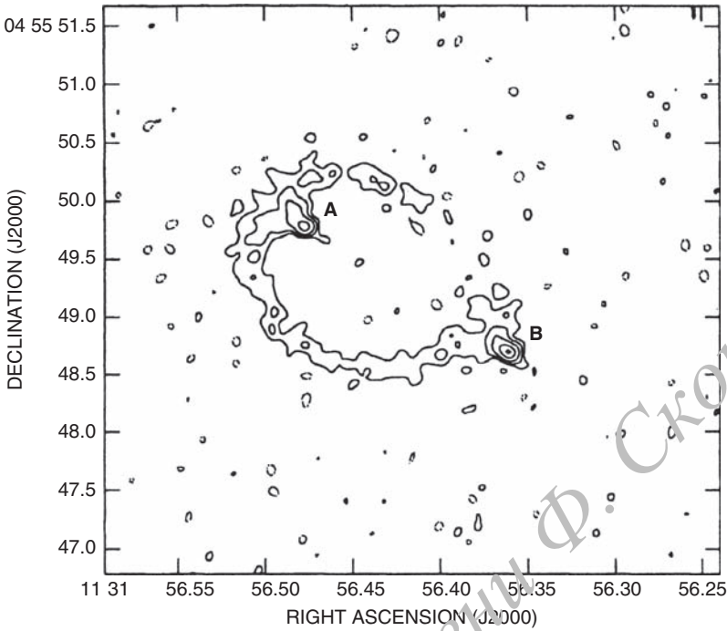
Fig. 13.6 A nearly complete Einstein ring MG 1151+0456 imaged at the radio frequency 15 GHz by the VLA (Very Large Array). From Chen and Hewitt (1993) . (©American Astronomical Society. Reproduced with permission from Astronomical Journal .)
