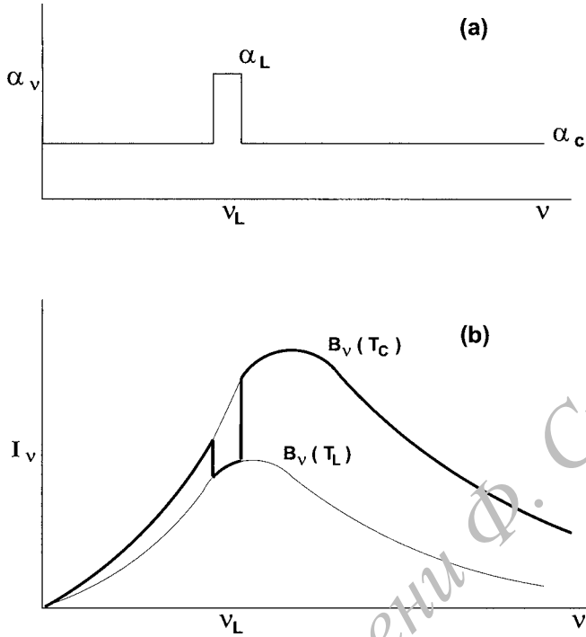
Fig. 2.7 For an absorption coefficient indicated in (a), the emergent spectrum is indicated in (b) by the dark line. The two blackbody spectra shown in (b) correspond to the temperatures T_C (upper curve) and T_L (lower curve) explained in the text.
