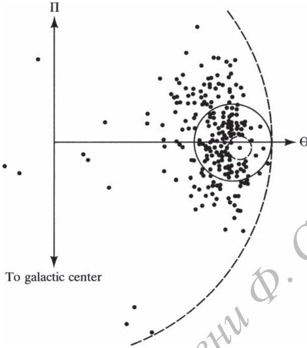
Fig. 7.5 A plot showing the values of \Pi and \Theta for stars in the solar neighbourhood. From Oort (1928).
