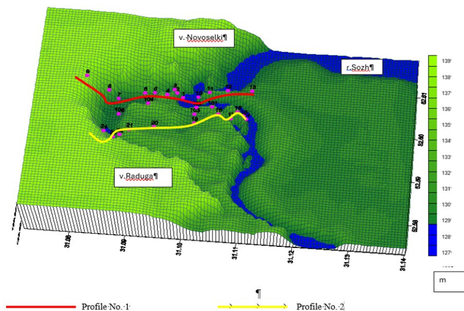
Figure 1 – Relief map of the study site
