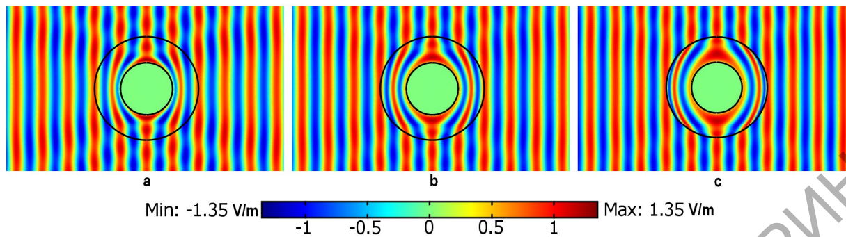
Fig. 1: E_z distribution for quadratic transformation based cloak. (a) \gamma=1.4 . (b) \gamma=1000 . (c) \gamma=-1.4 .
