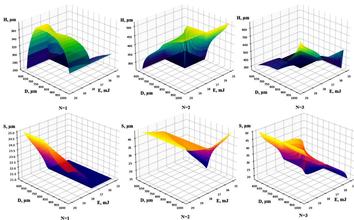
Figure 2.3 – Cavity depth H and width S as a function of processing parameters
